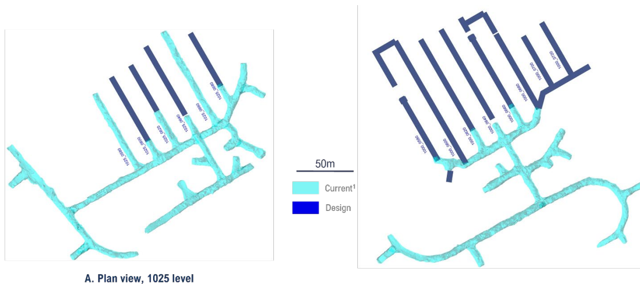
Figure 1: Plan view of 1025 level (A) and 1000 level (B) showing actual development (light blue) and planned development (dark blue) as at September 11, 2023.
